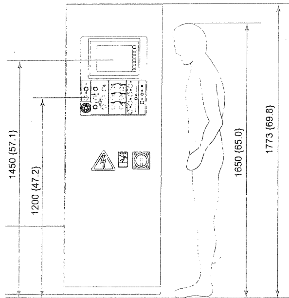
CONTROL BOX FRONT
