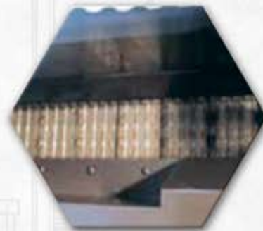
Chip conveyor system capable of removing cutting chips as well as access heat from sawing area.
